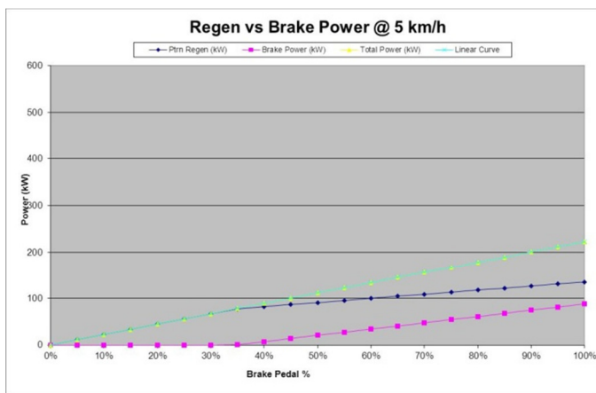
Figure 16 - Adaptive Regeneration at Low Speeds
