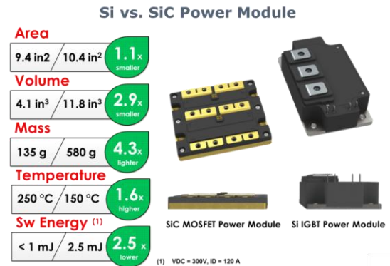
Figure 13. Comparison of HT-2000 high power (1200V and >100A) SiC power module with state-of-the-art Si-based power modules.
