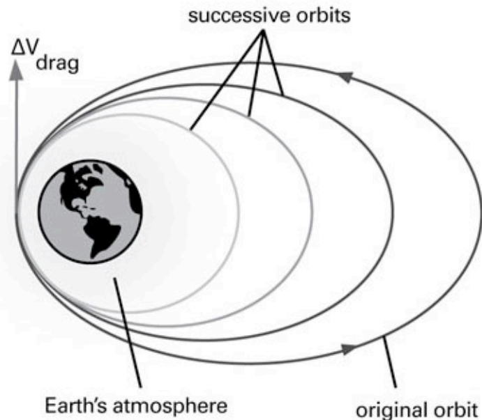
Figure 4–15. Effects of Drag on Eccentric Low Earth Orbit
