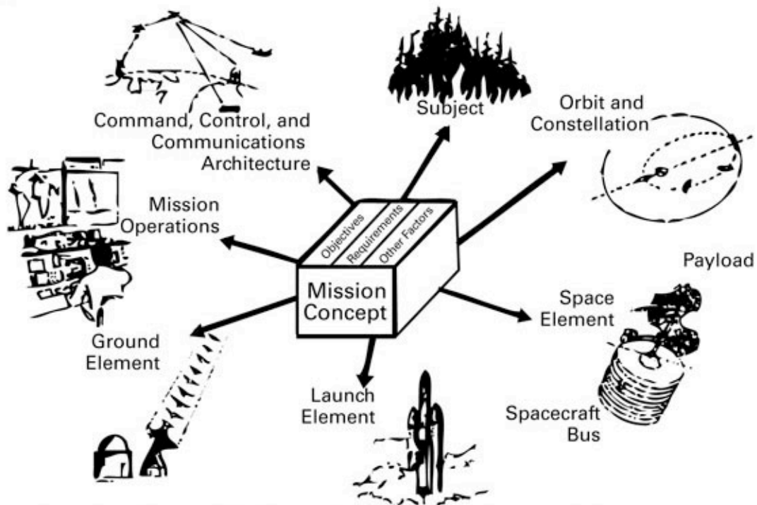
Figure 4–1. Mission Architecture
