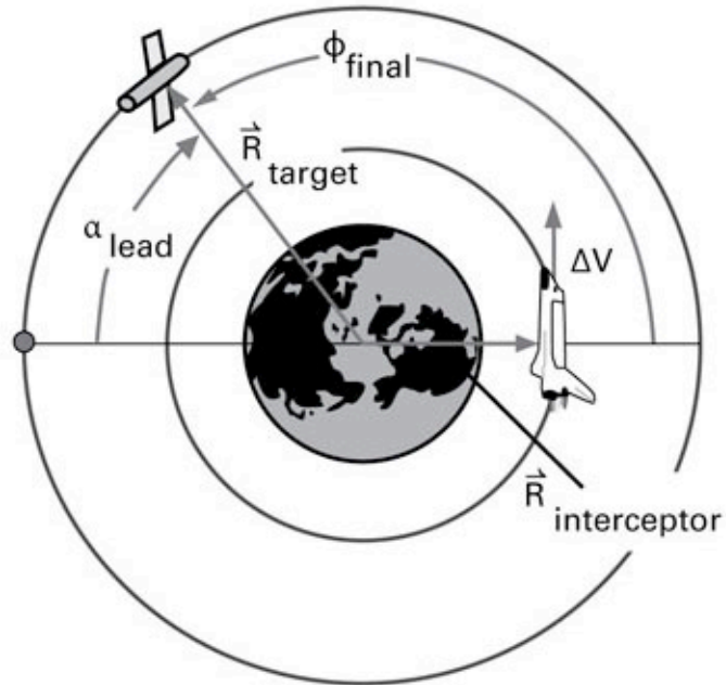
Figure 4–11. Coplanar Rendezvous
