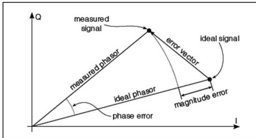
Figure 4. Vector Display of Modulation Errors (From [4])
