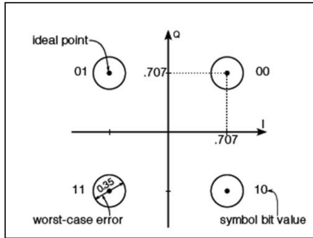
Figure 3. QPSK Error Shown on an I/Q Plane (From [4])
