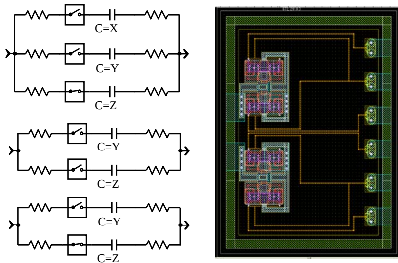
Figure 29: Circuit diagram for 3-bit and dual 2-bit tuners, and wafer-scale layout for dual 2-bit tuner.
