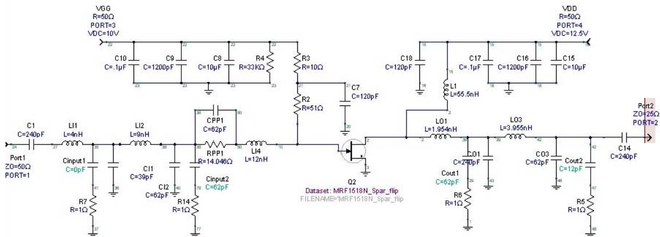
Figure 31: Revised model with greater detail on tuning circuit.
