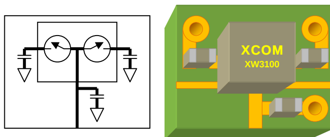
Figure 30: Architecture for remaining hybrid tuning circuit design
