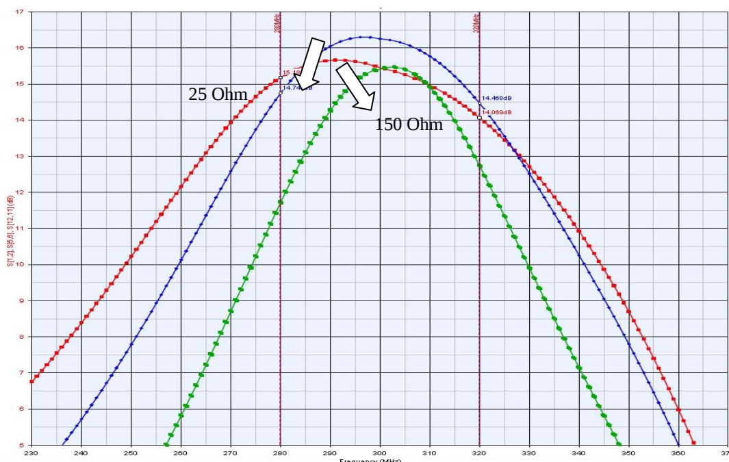
Figure 32: Amplifier de-tuning due to impedance mismatch with antenna.
