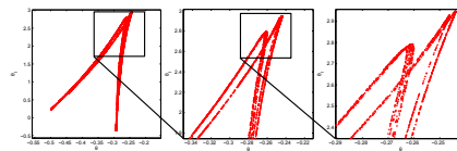
(c) Poincaré plots closeup
