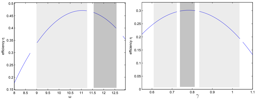
(c) Varying \omega - calculated efficiency
