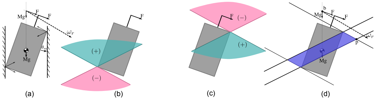
Figure 4.3: Ensuring jamming using the moment labeling method. (a) The contact friction cones are shown together with the resultant wrench \omega_r composed of m g and F . Figures (b) and (c) represent the nonnegative linear combination of the two lines of forces of the friction cone by moment labels. (d) The moment labeling representation of the composite wrench cone of contact forces the wall can apply to the mechanism. In this configuration, the resultant wrench \omega_r passes to the left of the (+) set, implying that this resultant wrench can be resisted by forces within the composite wrench cone of the contact forces and hence will stay jammed.
