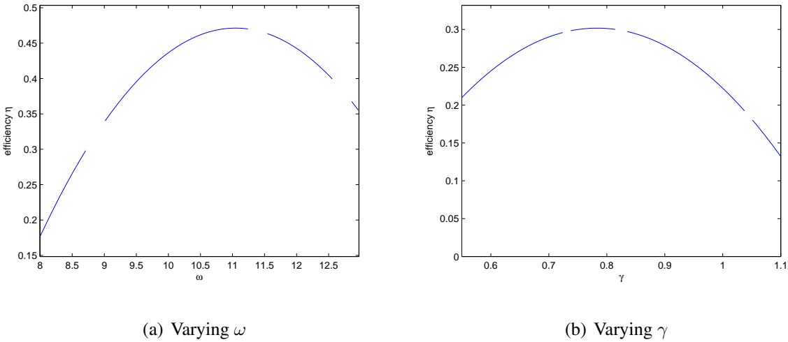
Figure 3.16: Efficiency calculation with change of input frequency \omega for parameters as in Figure 3.9(b) ((a)), and CoM location \gamma for parameters as in Figure 3.11(b) ((b)).
