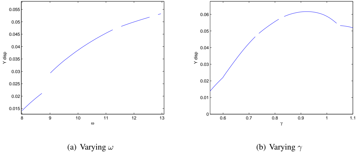
Figure 3.19: Averaged climbing rate with (a) change of input frequency ( \omega ) and (b) CoM location ( \gamma ).
