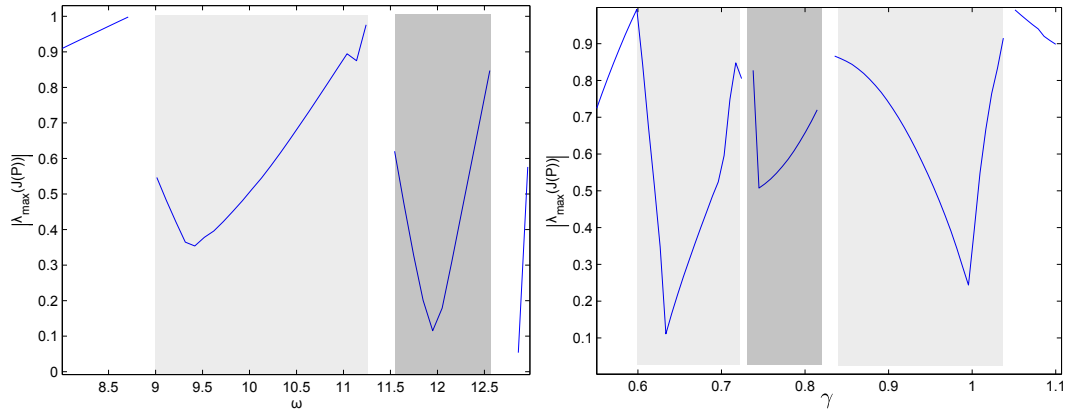
(a) Varying \omega - Max Lyapunov Exp.
