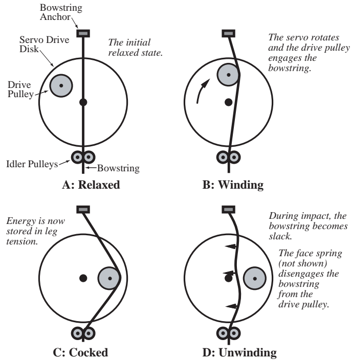
Figure 5.2: Schematic of the prototype thrust mechanism which stores energy in the leg during flight. The cycle begins in the relaxed state (A). During winding (B), the servo disk rotates, the drive pulley engages the bowstring, and the displacement of the bowstring compresses the leg (not shown). The energy stored in the cocked position (C) is a function of rotation angle. During the impact (D), the string goes slack, the face spring (not shown) nudges the bowstring off the pulley, and the leg extends to full length. Not shown are the servo body or the leg. The winding direction and string displacement alternate left-right. Reprinted from Brown and Zeglin (1998) ©[1998 IEEE].
