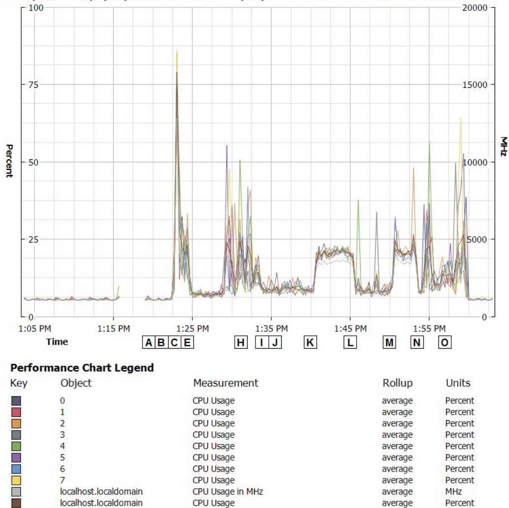
Figure 8. CPU Utilization of Physical Server #1.
