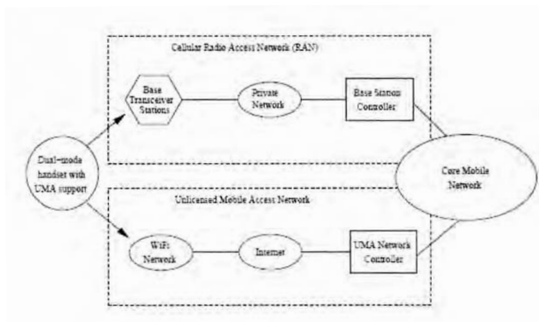
Figure 10.4. Unlicensed Mobile Access (UMA) Conceptual Architecture During a Call Setup.
