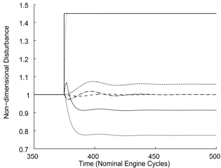
Figure 10 The response of the engine speed (---), brake torque (-·-·-), fuel flow rate (·····), and the pressure at the compressor outlet (-----), turbine inlet (-----) and turbine outlet (·····) to a step change in the back pressure (—)
