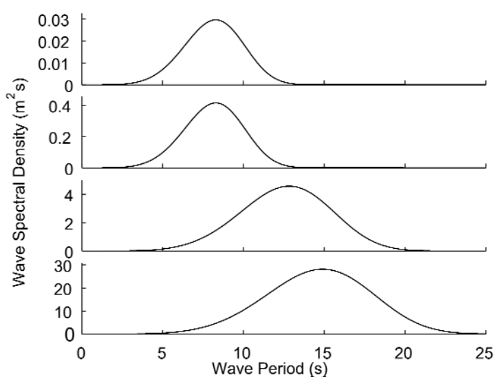
Figure 1 Bretschneider spectra representative of sea states 2, 4, 6 and 8. Note the different scales on the ordinates.
