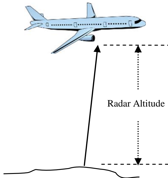
Figure 3-15: Radar Altimeter Concept.
