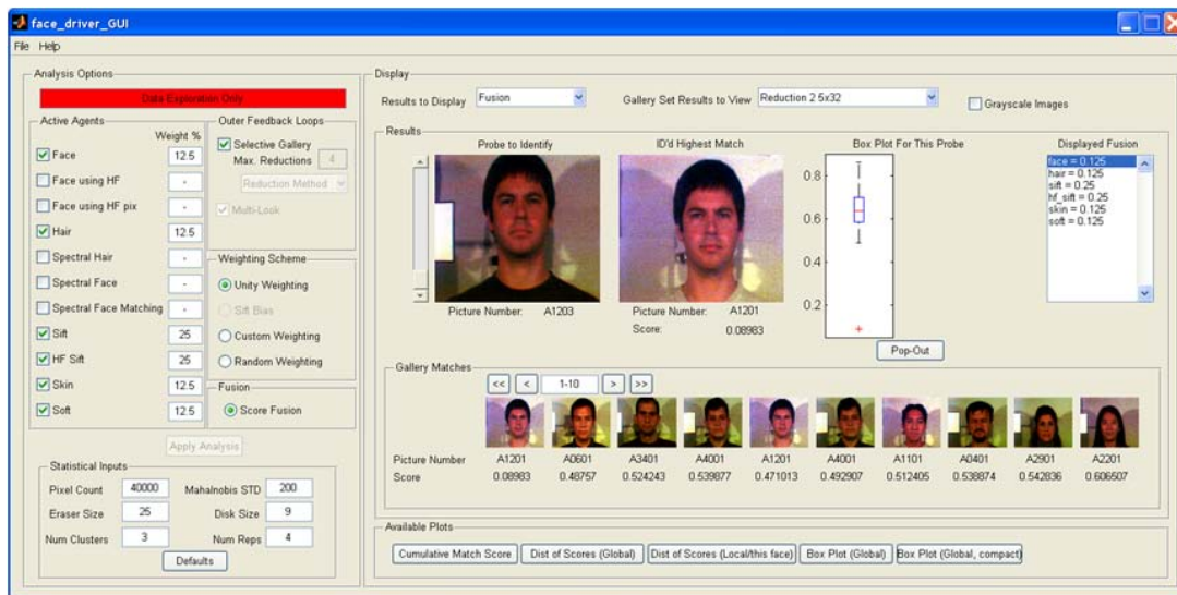
Figure 121: GUI Display for Second Reduction - Significant Improvement for Subject 12
