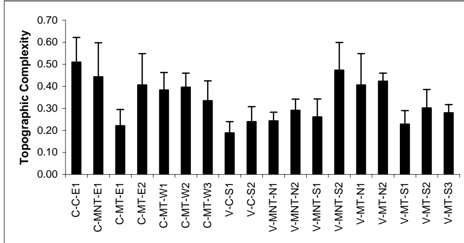
Figure 15. Topographic complexity of reefs at 18 study sites around Culebra (C) and Vieques (V) as determined from LPI transects (mean ± standard deviation, n = 6 assessments per site, except n = 4 for site V-MT-S2).
