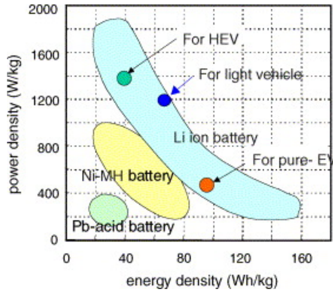
Figure 7: Battery Chemistries [38]
