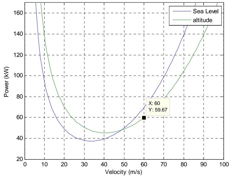
Figure 29: Hybrid Power Required Curve Cessna 172 Adjusted Performance
