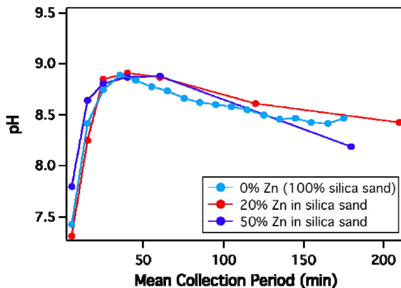
Figure 39. Effect of mass concentration of ZVZ in sand on column effluent pH over time. The pH appears to be independent of ZVZ concentration and therefore controlled by the sand not the ZVZ.
