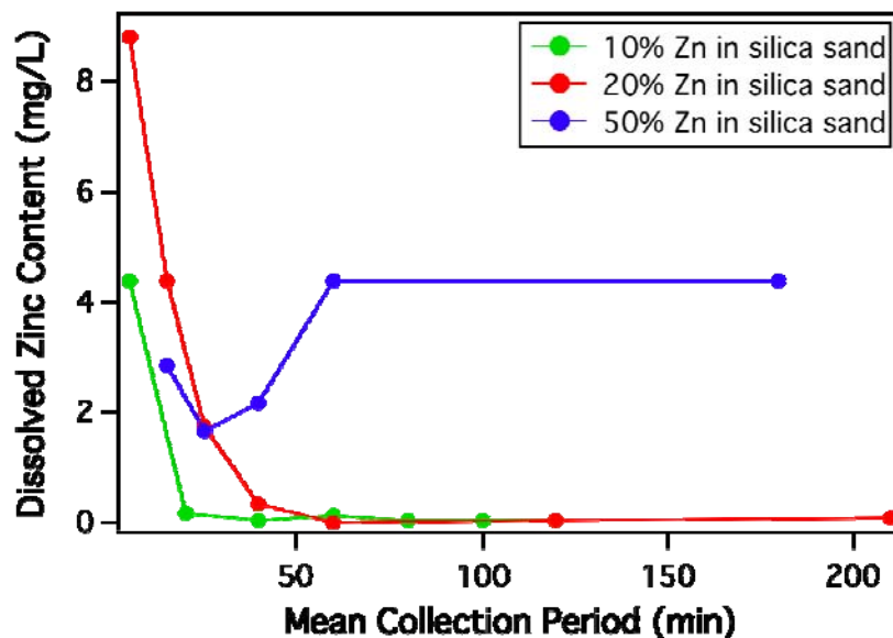
Figure 40. Effect of mass concentration of ZVZ in sand on effluent concentrations of Zn^{2+} over time.
