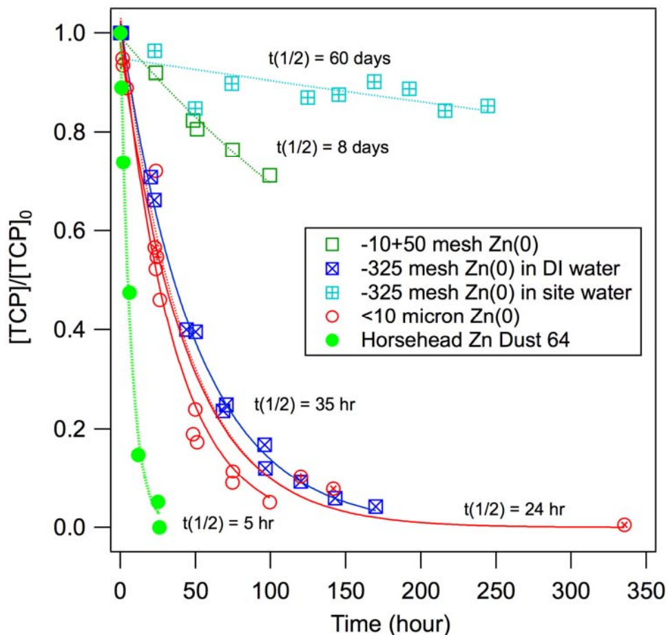
Figure 11. Kinetics of TCP disappearance with several types of reagent grade zero-valent zinc (ZVZ) in batch reactors made with deionized water or with a groundwater from an agricultural site in California. Replicates for the treatments shown in red and blue were deemed to be identical, so they were pooled and fit as one.
