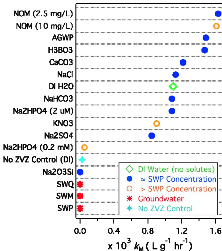
Figure 29. k_M values obtained from observed values shown in Figure 28 for TCP degradation by Zn64 in DI water, site groundwaters P, Q, and M, and various artificial groundwaters prepared at or above the concentration reported for Site Water P (SWP).
