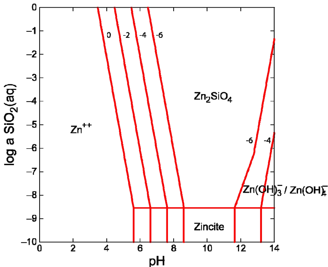
Figure 43. Predominance diagram for \text{Zn}^{2+} species in DI water as a function of \text{SiO}_2(\text{aq}) and pH. Lines shown represent equilibrium species transitions at [\text{Zn}^{2+}]_{\text{Total}} of 10^0 , 10^{-2} , 10^{-4} , 10^{-6} . It can be seen that, at \text{SiO}_2(\text{aq}) concentrations above 10^{-8.5} M (assuming \gamma = 1 ) zinc silicate ( \text{Zn}_2\text{SiO}_4 ) controls \text{Zn}^{2+} species solubility. Below 10^{-8.5} M, zincate ( \text{ZnO} ) controls \text{Zn}^{2+} species solubility.
