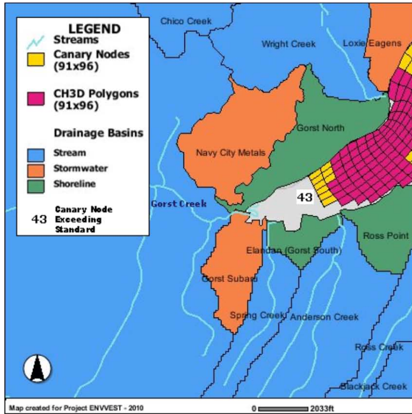
Map created for Project ENVVEST - 2010 WY2003-91x96: 43-Sin-Gorst-Creek30-Day Moving Geomean SURFACE
