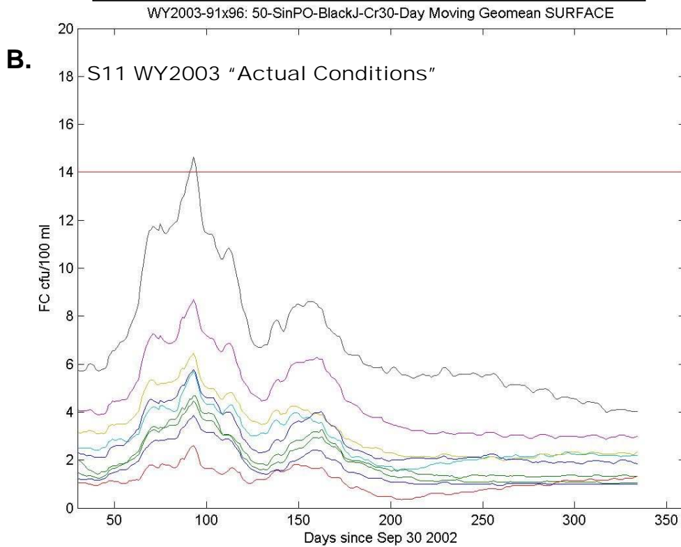
Figure 5-3. Location of Canary Node 50-SinPO-BlackJ-Cr (A) and simulated 30-day moving geomean for the surface grid cells (B) from simulation scenario S11 WY2003 "Actual Conditions."
