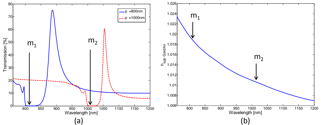
Fig.2. (a) Transmission spectra for 1-D- periodic arrays having p = 800 nm (blue line) and p = 1000 nm (red line). Two transmission minima ( m_1 and m_2 ) and band gaps are evident in the spectra. (b) Gold/air surface plasmon effective index dispersion: m_1 and m_2 are the wavelengths of the two minima in (a).
