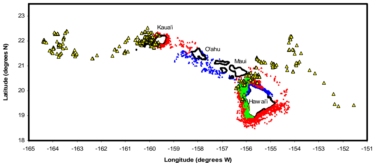
Figure 1. Map showing locations of satellite-tagged cetaceans tagged during June and July 2008. All individuals were tagged either off S.W. Kaua'i or W. Hawai'i. Species: false killer whales – blue; Blainville's beaked whales – green; short-finned pilot whales – red; melon-headed whales – yellow outlined with black. Some points overlap so that not all locations of some species (all except melon-headed whales) may be visible.
