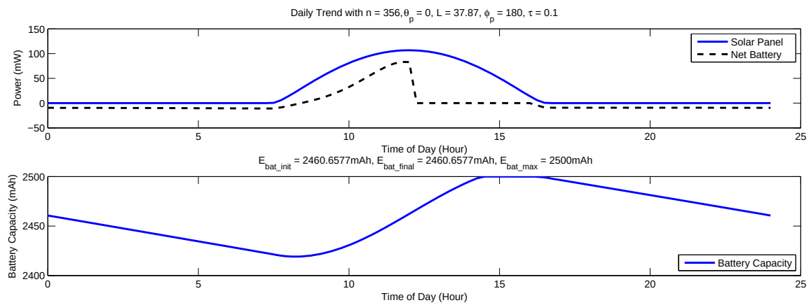
(c) Two 2500mAh NiMH batteries, I_{load} = 3.5mA
