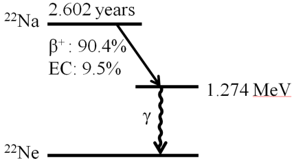
Figure 1.1. ^{22}\text{Na} decay scheme
