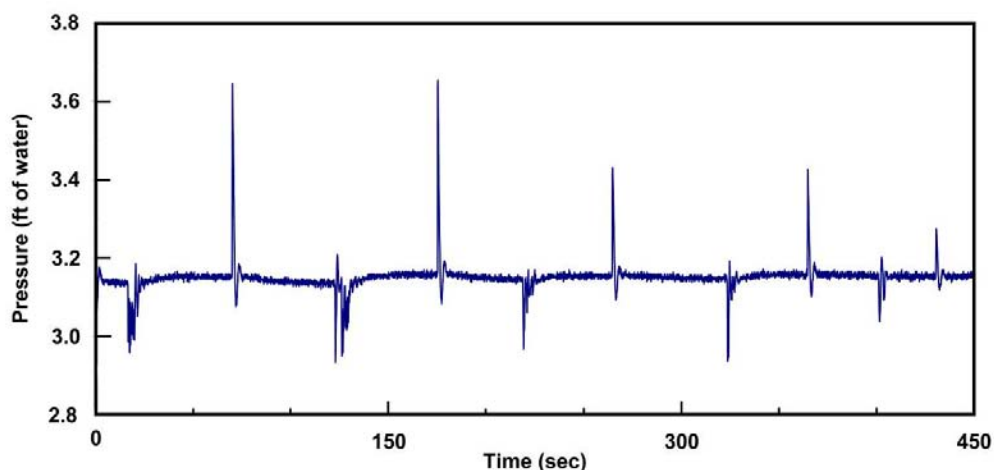
Figure 6a. Plot of falling-head tests conducted in this well. Pneumatic slug tests were performed using an inflatable packer system with schedule 80 nominal ½-in. polyvinyl chloride (PVC) riser. The first two tests had H_o of approximately 20 in. of water displacement. The third and fourth tests had H_o of approximately 10 in., and the fifth test had H_o of approximately 5.0 in. of water displacement. Note that the transducer-observed pressure on the first two tests is only about 0.6 ft. This is about 30% of the 20 in. of water pressure observed on the pressure gauge of the pneumatic head. The other slug tests show a similar reduction of transducer pressure as compared to the gauge pressure for this series of tests. In general, the transducer-observed pressure is always somewhat less than the ideal H_o pressure applied for slug tests. This phenomenon is due to several factors and is the topic of current and ongoing research. The tests shown here are extreme examples of this behavior.
