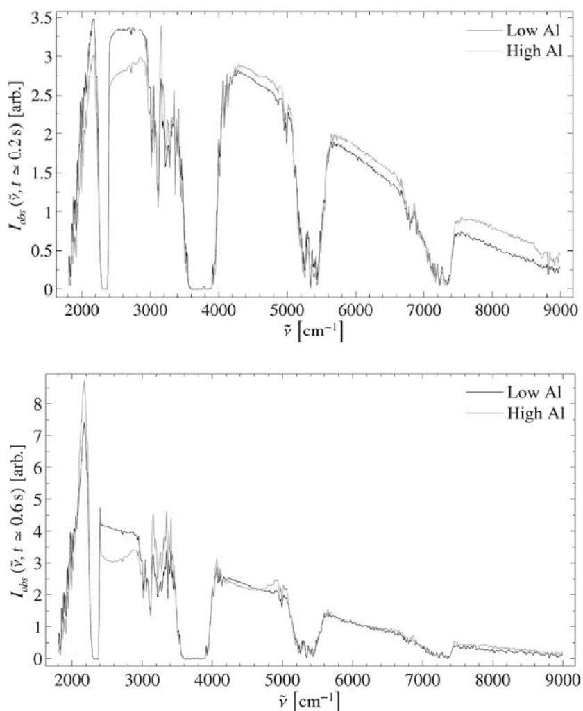
Figure 5. Normalized spectra corresponding to RDX containing low (—) and high (---) aluminum content at (top) 0.2 s and at (bottom) 0.6 s. At early times, both spectra are dominated by continuum radiation from the soot. As time progresses, the high-Al RDX exhibits more selective emission near 2100, 3200, and 4950 \text{cm}^{-1} .
