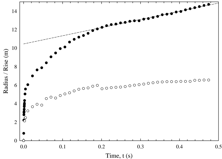
Figure 18. Temporal evolution of the fireball: (○) radius and (●) left height at longer times. The fireball rise begins to approach a constant rate beginning at approximately 0.25 s.
