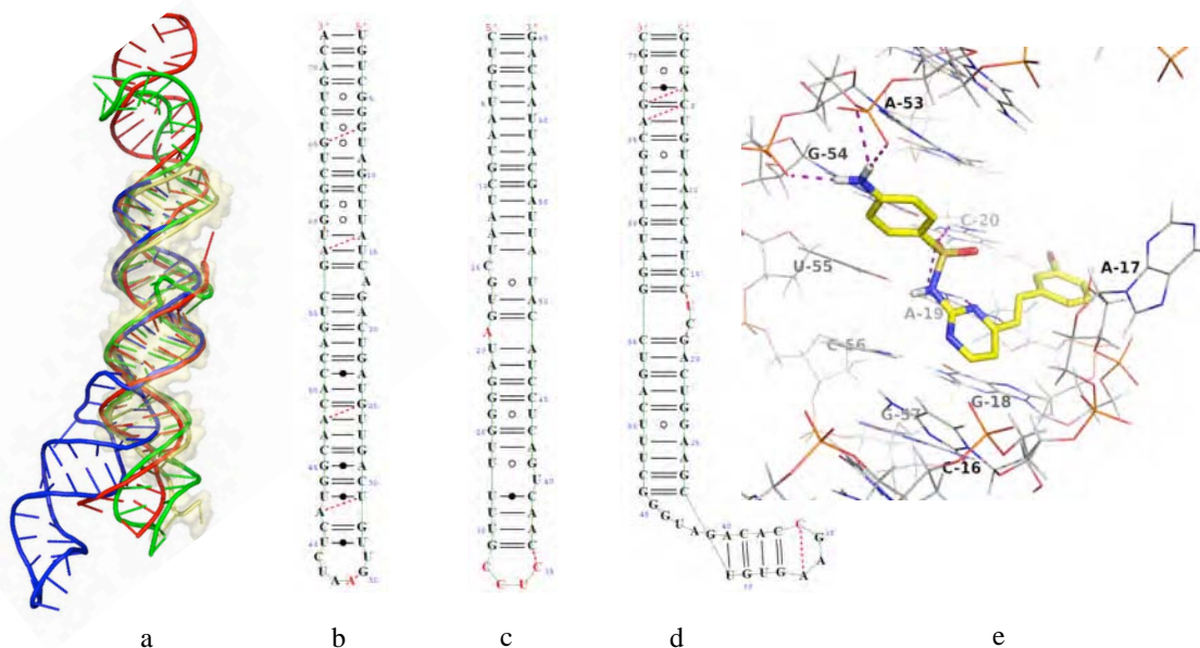
Fig. 1. pre-miR-21, pre-miR-155 and pre-miR-30a structural models and binding pose of one hit. a. Superimposition of MC-Fold/MC-Sym predicted pre-miR30a (green), pre-miR21 (red) and pre-miR155 (blue) on pre-miR30 crystal structure 3A6P (yellow). b-d. Illustration of secondary features observed from 3D models depicted by RnaxmlView. miR-21 (b); miR-155 (c); miR-30a (d). e. Predicted hit binding pose.
