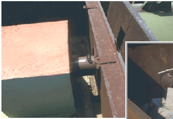
Test Setup Prior to Water Fill
