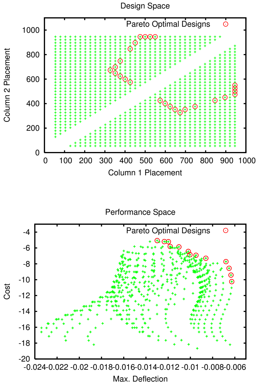
Figure 3.3: Pareto optimization in the 2D bridge design study. Pareto-optimal points are circled in red.
