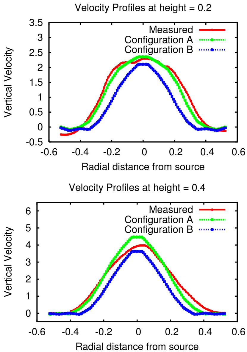
Figure 3.10: Comparing the velocity profiles of two input configurations at two heights.
