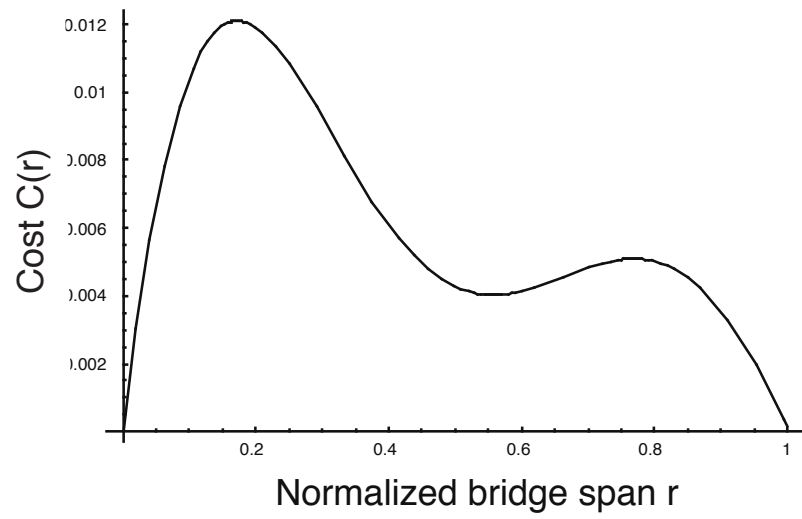
Figure 3.2: Support cost as the function of the distance to the left endpoint.
