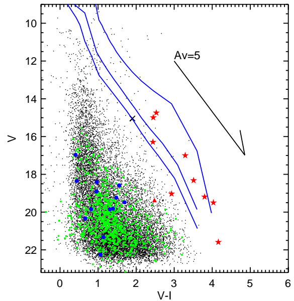
Figure 5. Optical V vs. V - I_c color-magnitude diagram. The symbols are the same as in Figure 4. Note that the blue dots representing the [3.6] > 12 sources are in fact plotted, but they are amongst the green squares and black dots well below the zero-age main sequence (ZAMS); this we take to be further evidence that the objects represented by the blue dots are contaminants and not YSO candidates. The red triangle is the edge-on disk candidate, which appears here below the ZAMS, as appropriate for such an object. The solid blue lines are models from Siess et al. (2000) at 1, 10, and 30 Myr and scaled to 210 pc, where we have tuned the color-effective temperature relation such that the 100 Myr isochrone matches that of the Pleiades single-star sequence (Stauffer et al. 2007; Jeffries et al. 2007). A reddening vector is also indicated.
