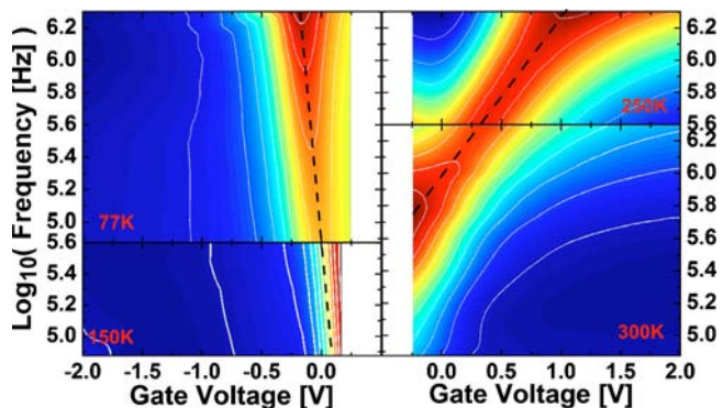
FIG. 2. (Color online) Conductance ( G/\omega ) contours of n-type and p-type GaSb MOSCAPs with PEALD \text{Al}_2\text{O}_3 showing good Fermi level modulation toward valence and conduction band sides.
