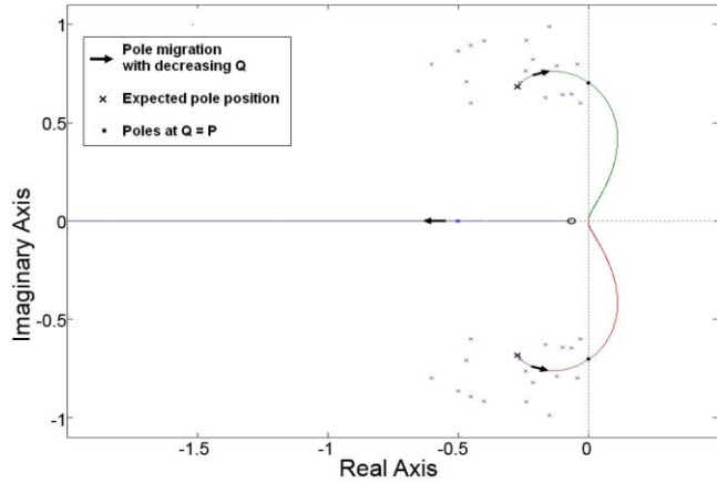
Fig. 13. Shifted mass step response pole positions.
