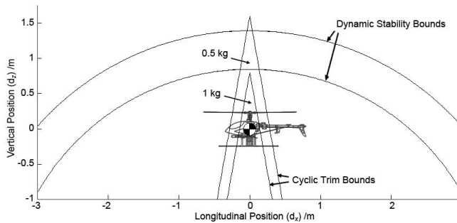
Fig. 9. Position stability bound isoclines for 0.5 and 1 kg loads.
