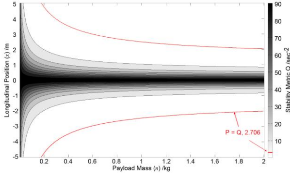
Fig. 5. Stability metric position-mass isoclines, d_z = 0.2\text{m} .
