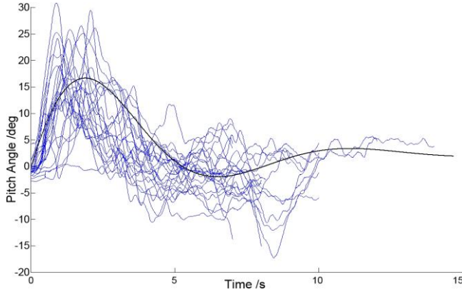
Fig. 12. Shifted mass step responses
