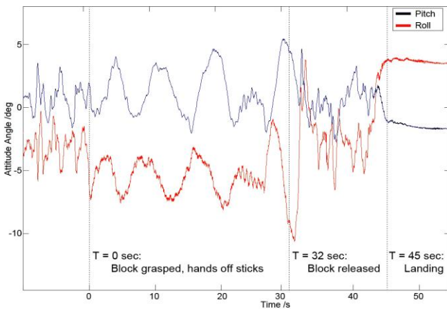
Fig. 16. Coupled hovering pitch and roll angles.
