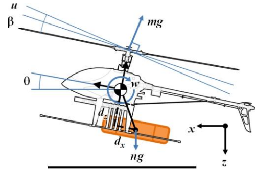
Fig. 3. Planar aircraft dynamics free body diagram.
