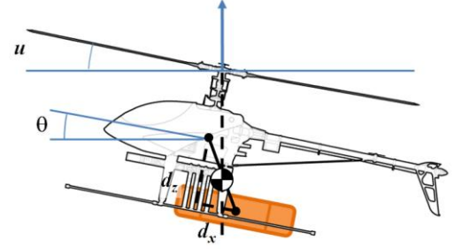
Fig. 7. Cyclic trim balance angle
