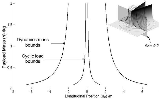
Fig. 8. Longitudinal position-mass stability bounds for d_z = 0.2 m.
