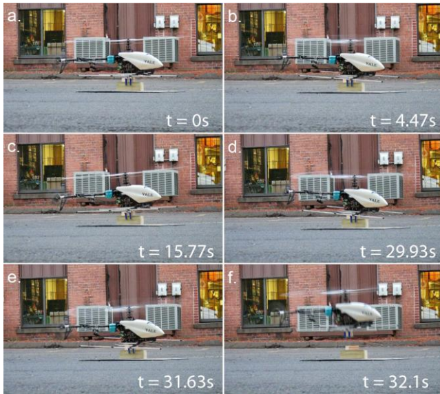
Fig. 15. Coupled hovering, grasping a block fixed to ground
