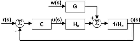
Fig. 6. System Disturbance Block Diagram.
