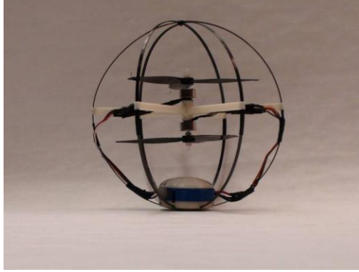
Figure 14. Assembled rotochute side view.
