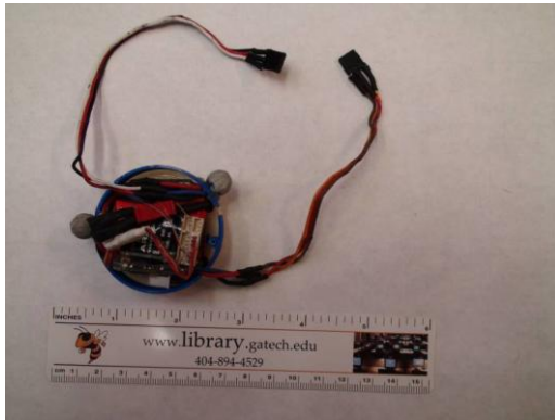
Figure 9. Combined base and wiring harness.
