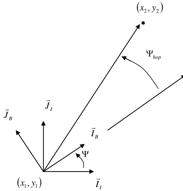
Figure 15. Angle definition for micro hopping rotachute controller.
