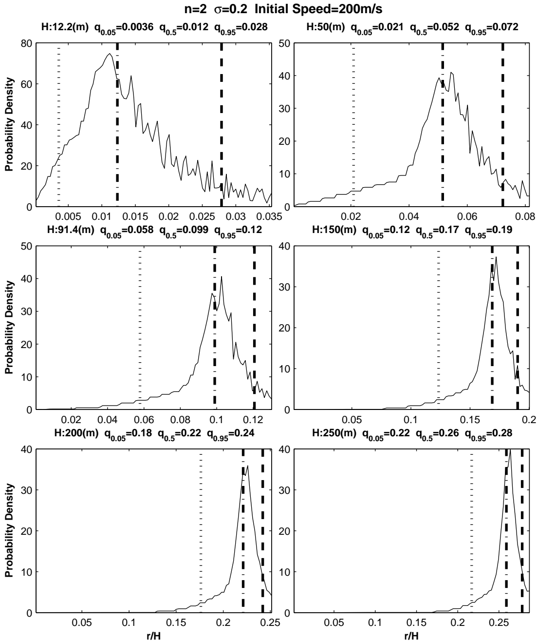
Fig. 11. Probability distribution of the bomb's horizontal drift (scaled by the depth) r/H with n = 2 , \sigma = 0.2 , V = 200 m/s for various depth: (a) 12.2 m (i.e. 40 ft), (b) 50 m, (c) 91.4 m (i.e., 300 ft), (d) 150 m, (e) 200 m, and (f) 250 m.
