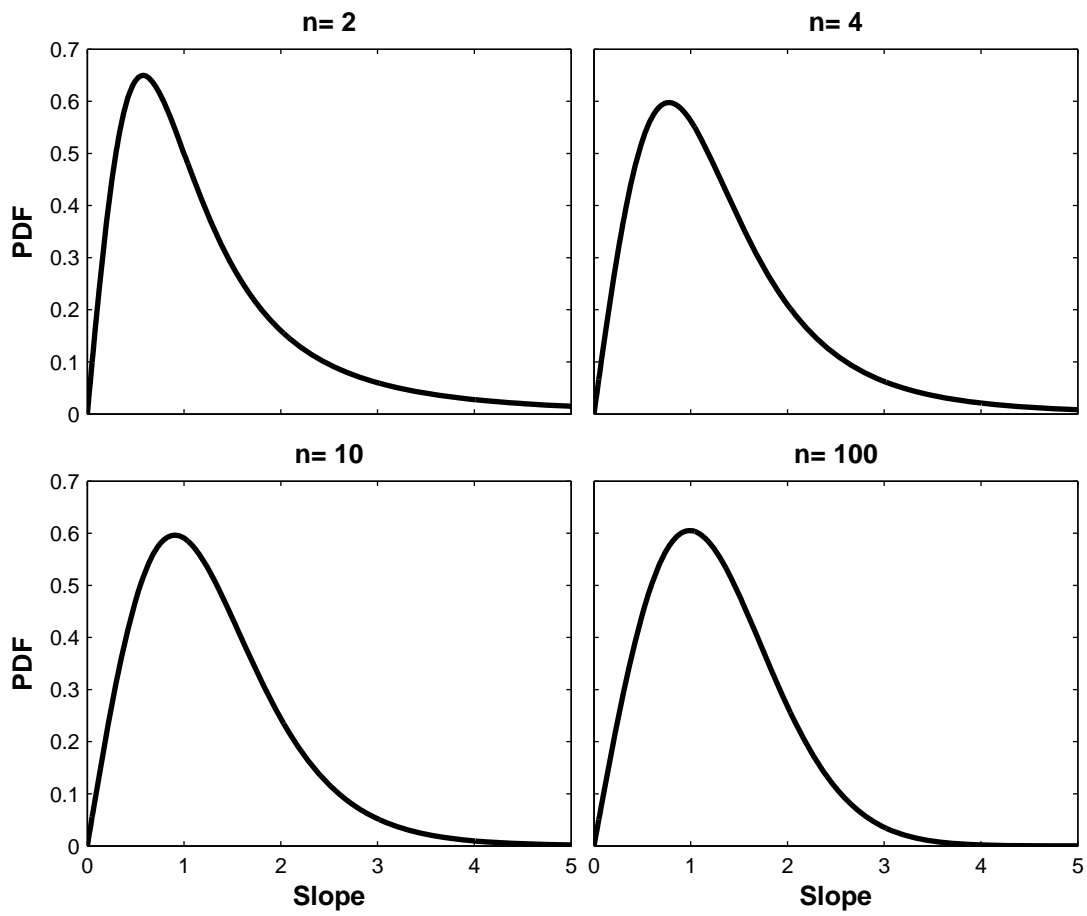
Fig. 6. The s-PDFs for various surface characteristics: (a) n = 2 , (b) n = 4 , (c) n = 10 , and (d) n = 100 .
