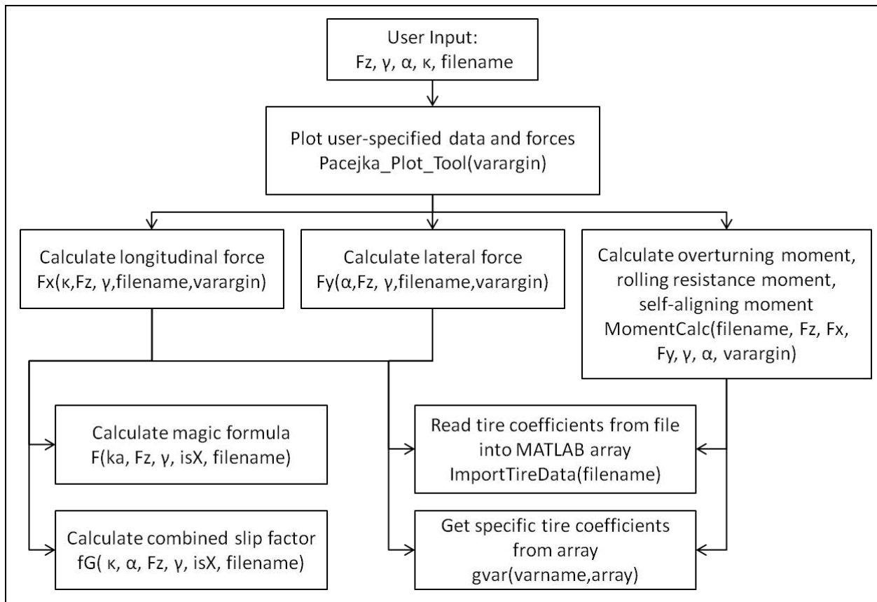
Figure 3 – Interaction of MATLAB files
