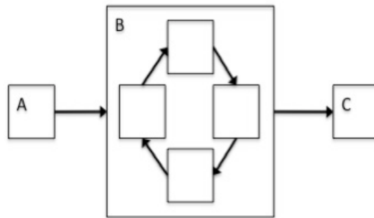
Figure 2. Acyclic Flows with Policy Equivalence Class
