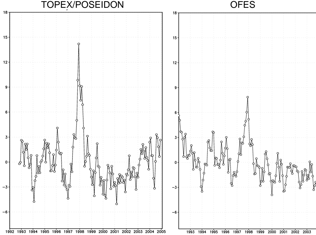
Figure 5. Monthly SSH variance from between the equator and 18^{\circ}\text{N} and from 40^{\circ}\text{E} to 60^{\circ}\text{E} from Topex/Poseidon (left) and the OFES hindcast run (right). Note the extreme low in the spring of 1994 and the extreme high SSH in the spring of 1998. Both extrema are seen in the OFES simulation.
