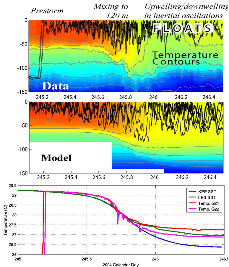
Figure 1: (top) shows Temperature (contours and floats) from EM and Lagrangian floats G21 and G22 (Sanford, D’Asaro) overlaid with Hurricane Frances Lagrangian float observations. (middle) corresponding LES model with floats (middle), vs. time and depth (m). Model float depth distributions and vertical T agree well with the data. Proper prediction of mixed layer depth changes will require further specification of upwelling due to larger scale dynamics, but LES sea surface temperature (bottom) compare well with Lagrangian float G22. An LES equivalent column model based on KPP matches LES evolution as the wind rises but predicts significantly more entrainment and cooling as wind drops and compares less favorably with observations.
