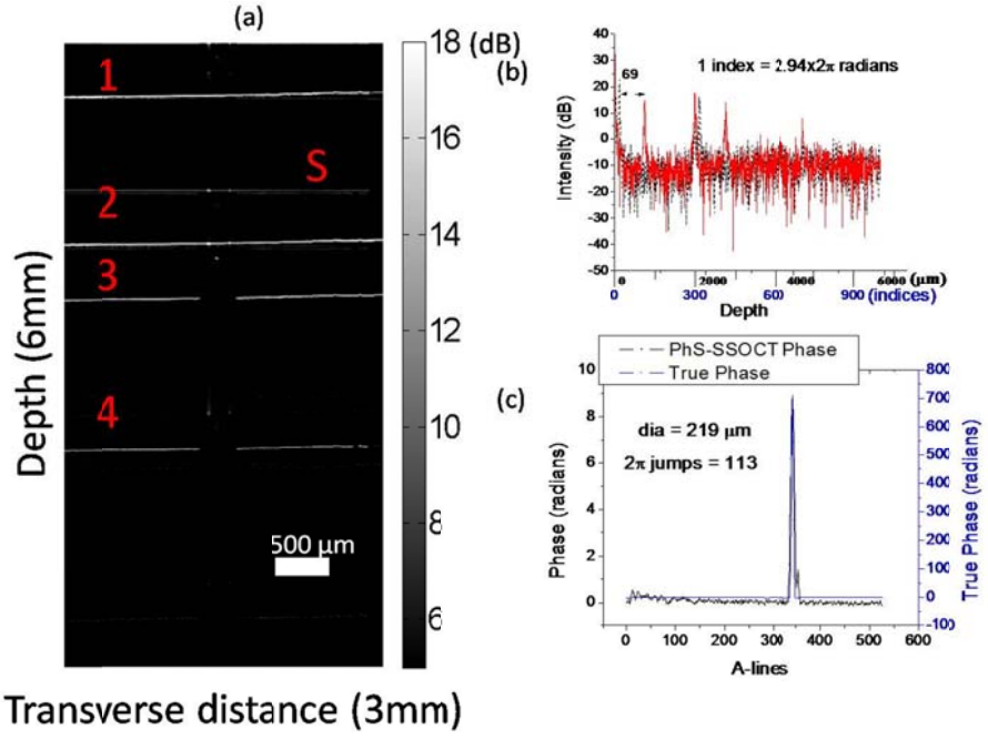
Figure 8: (a) Image of a cuvette of 500 μm thick containing a bubble of 224 μm (1,2,3,4 are the surfaces corresponding to 1,2,3,4 in figure 4(a) and S is the self-interference image) (b) corresponding 1-D profile showing the bubble induced shift in peak (c) temporal phase response at 665 μm peak.
