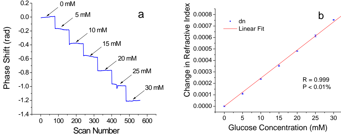
Figure 5: (a) Phase shift measured in a clear aqueous solution of glucose vs. time (or scan number); and (b) change in the sample's refractive index as a function of glucose concentration.
