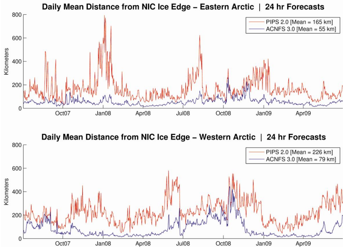
Figure 9. Regional daily mean distances (km) from the NIC observed ice edge locations to the ice edge location using the 24 hr forecasts from ACNFS (20%-blue) and PIPS 2.0 (20%-red) for the eastern Arctic (top) and the western Arctic (bottom) during July 2007 – June 2009.
