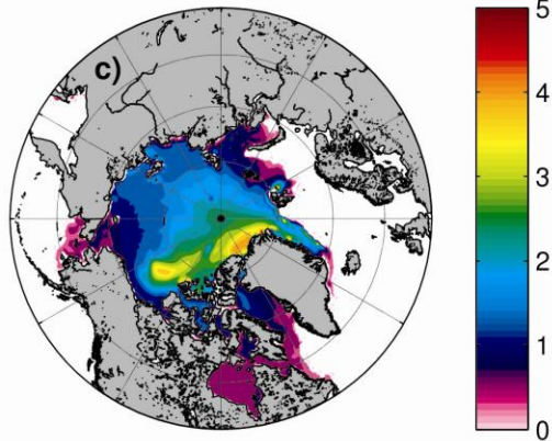
PIPS 2.0 Ice Thickness (m) | 2008 12 29
