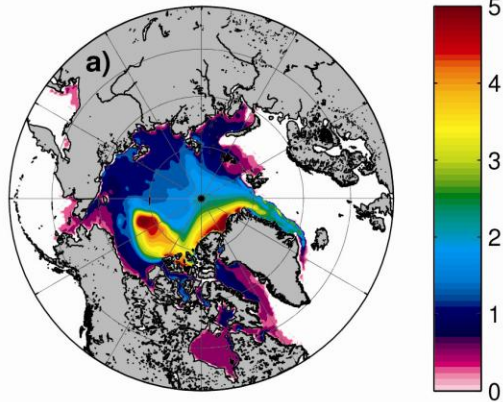
PIPS 2.0 Ice Thickness (m) | 2007 12 29
