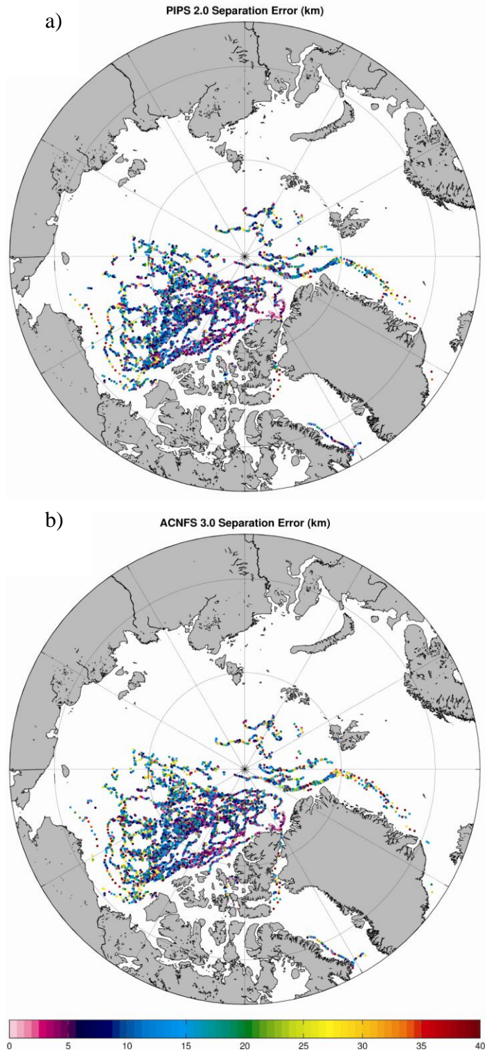
Figure 21. 24 hr separation error (km) from a) PIPS 2.0 and b) ACNFS for each Argos buoy position.
