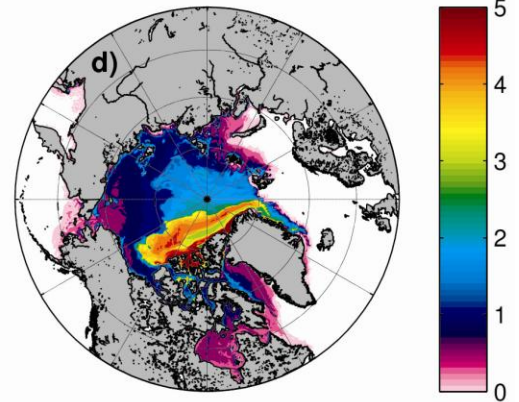
ACNFS 3.0 Ice Thickness (m) | 2008 12 29
