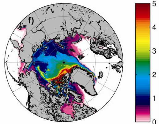
Figure 7. Ice thickness (m) snapshots from PIPS 2.0 (left) versus ACNFS (right). Top panel is from 2007, middle is 2008 and bottom panel is 2009 valid for 29 December.
