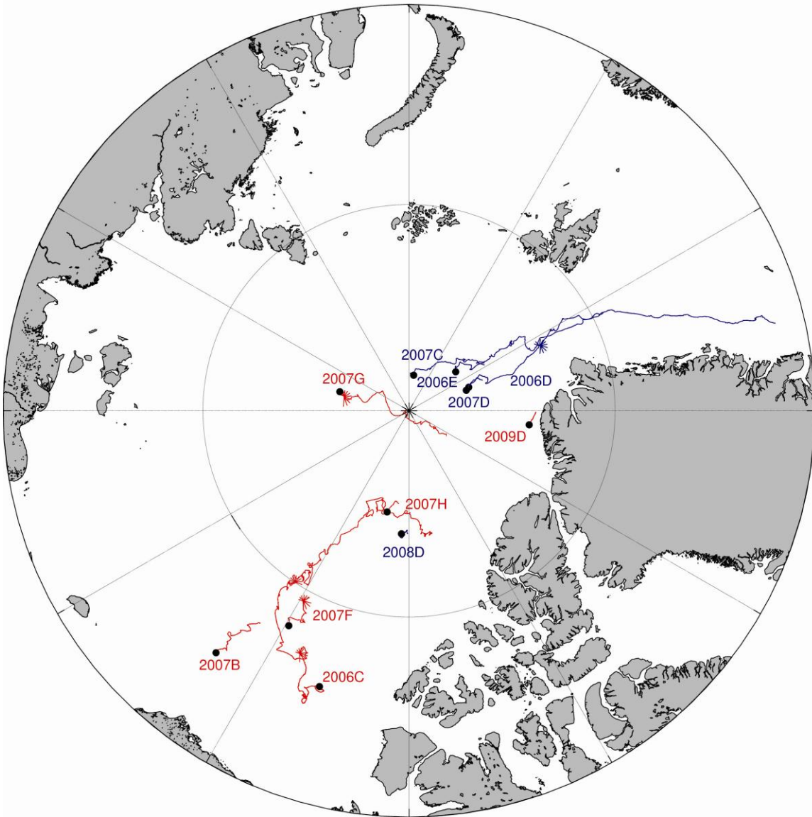
Figure 11. Drift paths of IMB from July 2007 – May 2009. A black circle indicates the starting position of each buoy. For the tracks in blue, the ACNFS produced lower ice thickness errors; for the tracks in red, the PIPS 2.0 produced lower ice thickness errors.
