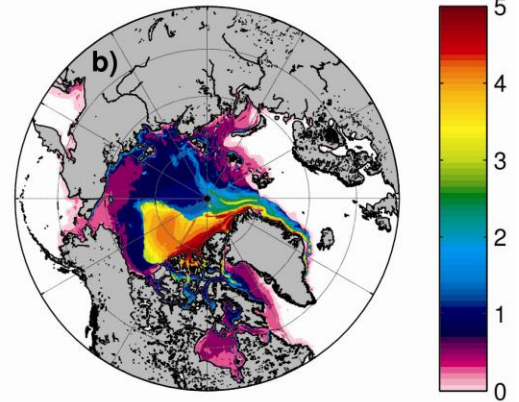
ACNFS 3.0 Ice Thickness (m) | 2007 12 29
