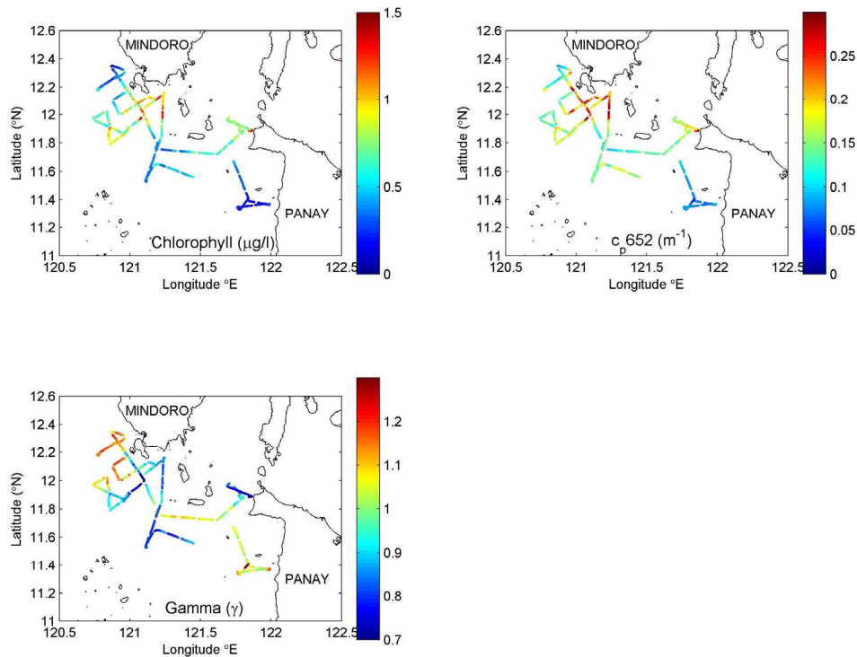
Figure 4. Near-surface underway distribution of chlorophyll concentration, beam attenuation ( c_p652 ) and the gamma-c (slope of beam attenuation coefficient as a function wavelength). Low gamma values indicate larger particle size and larger gamma values indicate smaller particle size distribution.
