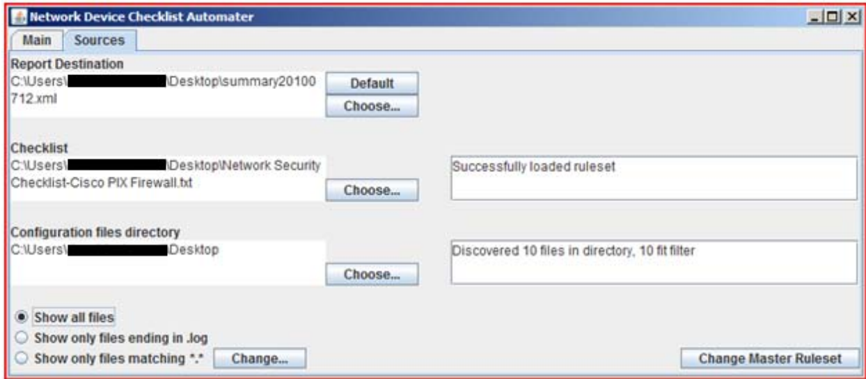
Figure 6. Sources tab with options selected.
