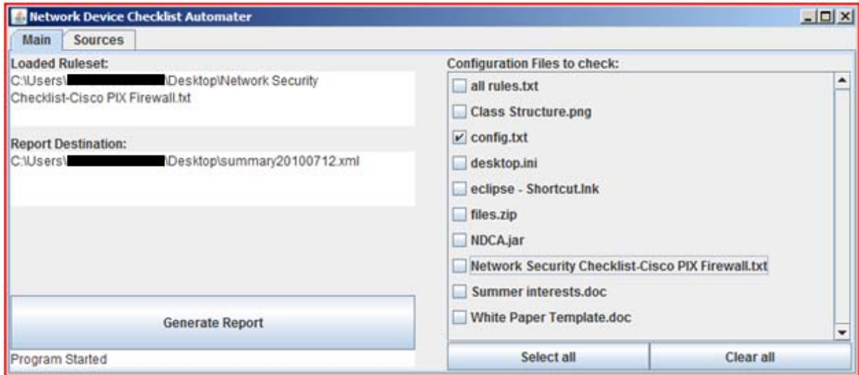
Figure 8. Main screen with options selected, ready to run.
