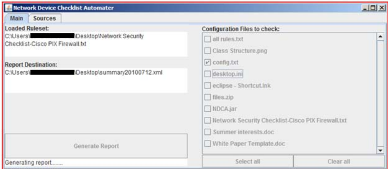
Figure 9. Main screen while generating a report.
