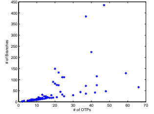
Fig. 10. This figure shows the relationship between the OTP set size, along the x-axis, and the number of branches in the search tree, along the y-axis, for the road network data.
