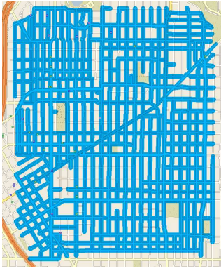
Fig. 8. This is the road network we used as our real-world example. This network covers an area of 1.5 miles by 2 miles. The edges and nodes included in our graph are highlighted in blue.
