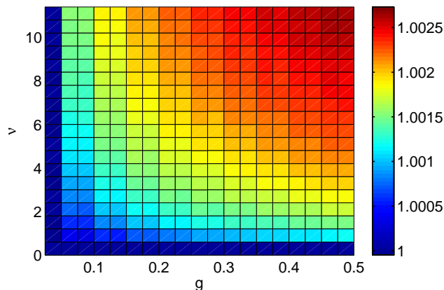
Figure 7: Extinction factor increase as a function of vaccination parameters numerically computed using the Monte Carlo simulation. Parameters shown are g =vaccination amplitude (percentage of susceptibles) and \nu =vaccination frequency per year. The population size is N = 1000 .
