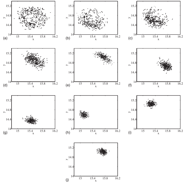
Figure 2: Snapshots of a swarm taken at (a) t = 50 , (b) t = 60 , (c) t = 62 , (d) t = 64 , (e) t = 66 , (f) t = 68 , (g) t = 70 , (h) t = 72 , (i) t = 74 , and (j) t = 76 , with N=300 particles, and noise intensity, D=0.08 . The swarm was in a rotational state when the time delay of 1 was switched on at t = 40 .
