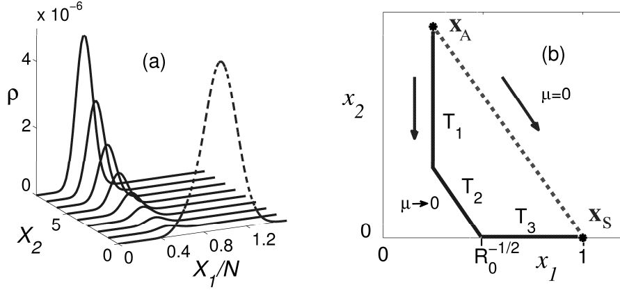
Figure 5: A snapshot of the probability \rho(\mathbf{X}) near the extinction plane X_2 = 0 for the SIS model; \rho is quasi-continuous in X_1/N , with X_1 and X_2 being the total numbers of susceptibles and infected, respectively, and N being the characteristic total population. The data of simulations refer to \mu t = 9, R_0 = 4, \mu' \equiv \mu/(\mu + \kappa) = 0.1 , where \mu is the birth-death rate and R_0 is the infection reproduction rate. For t = 0 the system was at the stable state \mathbf{X}_A , the total number of particles was N = 50 . (b) Asymptotic optimal trajectories for extinction for \mu \rightarrow 0 (solid line) and \mu = 0 (dashed line).
