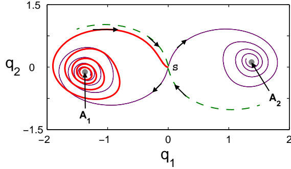
Figure 4: Phase portrait of a two-variable system with two stable states A_1 and A_2 . The saddle point \mathcal{S} lies on the separatrix that separates the corresponding basins of attraction. The thin solid lines show the downhill deterministic trajectories from the saddle to the attractors. A portion of the separatrix near the saddle point is shown as the dashed line. The thick solid line shows the most probable trajectory that the system follows in a fluctuation from A_1 to the saddle. The most probable switching path (MPSP) from A_1 to A_2 is comprised by this uphill trajectory and the downhill trajectory from \mathcal{S} to A_2 . The plot refers to the system studied experimentally, an underdamped nonlinear parametrically modulated oscillator with the modulation frequency close to twice the eigenfrequency.
