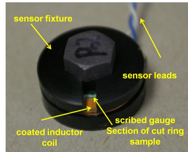
Assembled sensor
