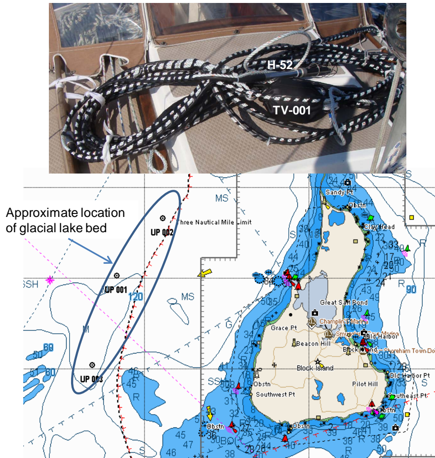
Figure 6: Hybrid vertical array and target geoacoustic feature.
