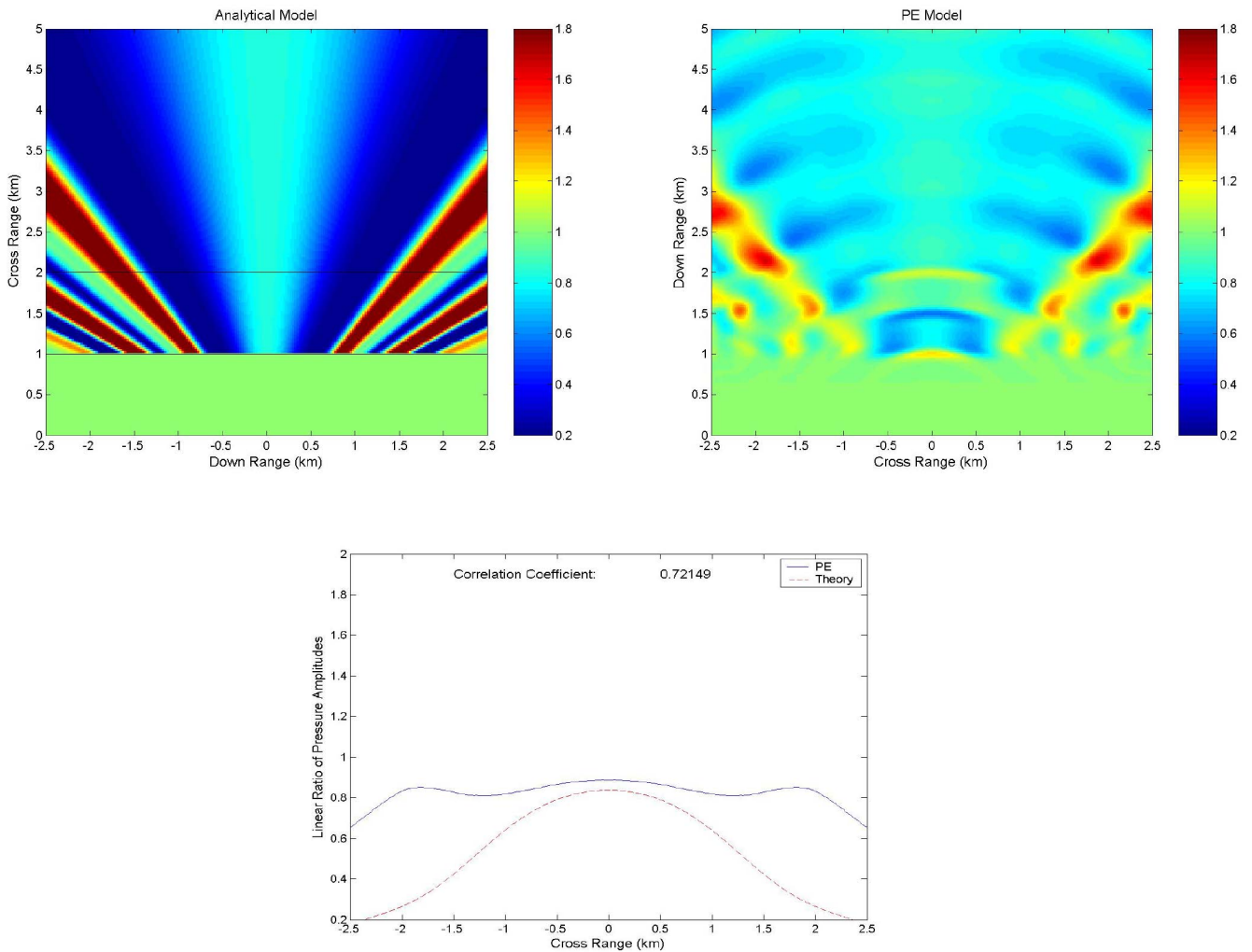
Figure 3: Comparison of ratio of modal energies between single-scattering model solution (upper left figure, red curve below) and 3-D MMPE solution (upper right figure, blue curve below) for mode 5 at 150 Hz. Lower figure shows comparison at 5 km range.
