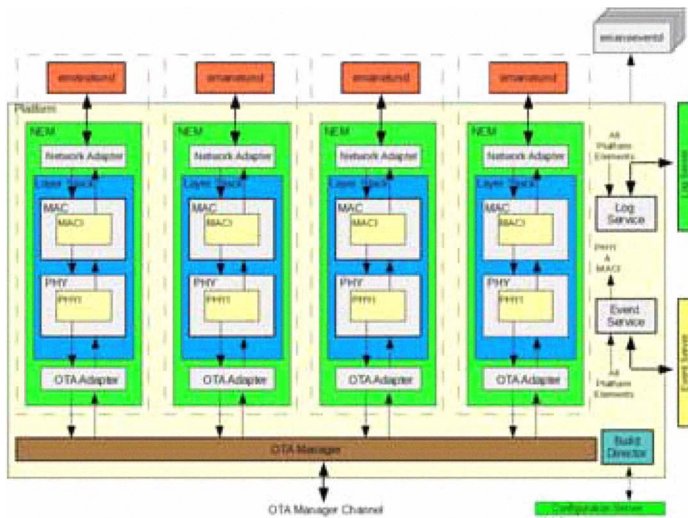
Figure 1 – eMANE Architecture
