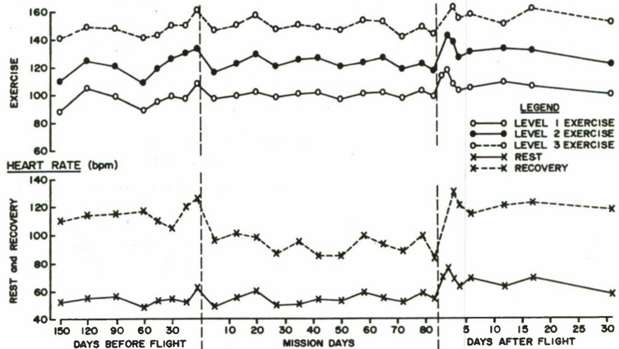
Fig. III-9. Heart rate, Skylab 4 Pilot. (Modified from ref. III-19. p. 736.)
