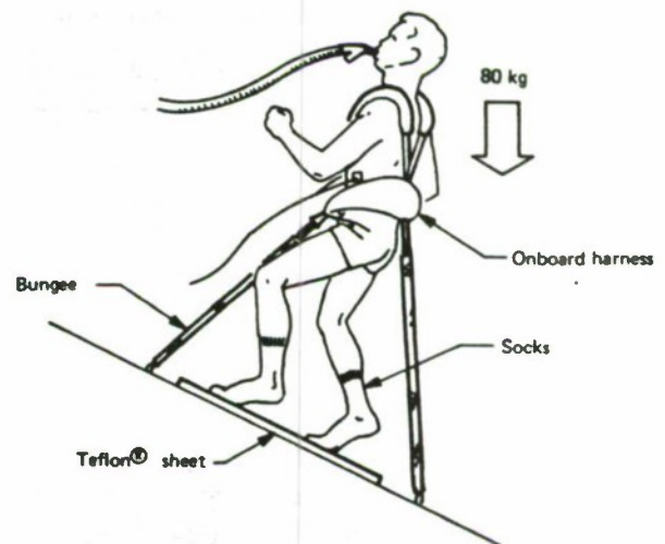
Fig. III-13. Treadmill arrangement. (From ref. III-24, p. 411.)
