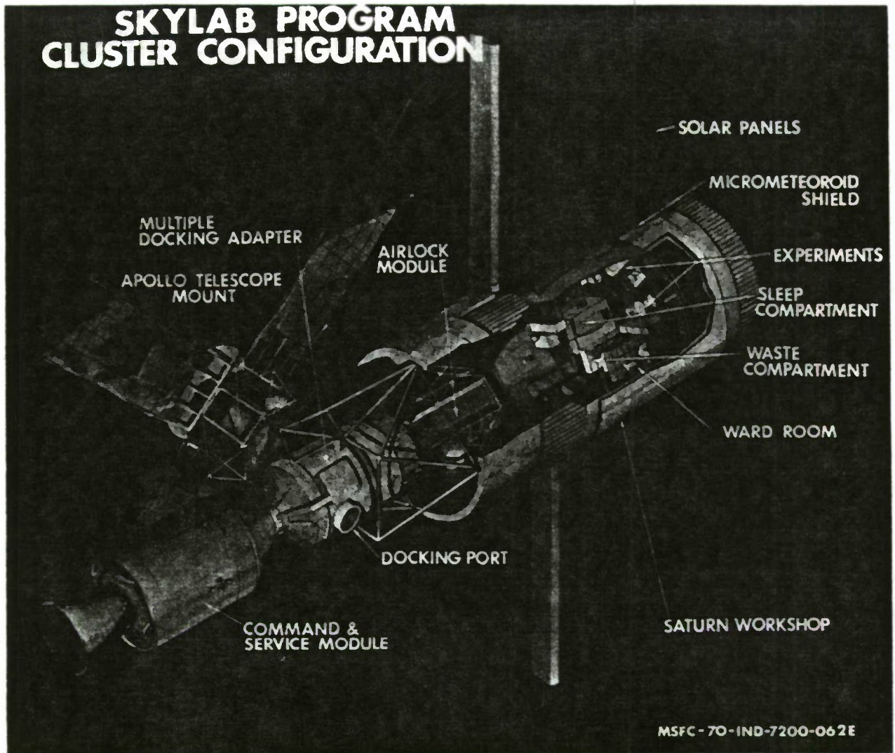
Fig. II-2. The deployed Skylab cluster.
