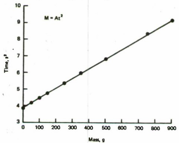
Fig. II-5 (b). Calibration curve Skylab 2 small mass measuring device, mission day-9. (From ref. II-12, p. 375.)
