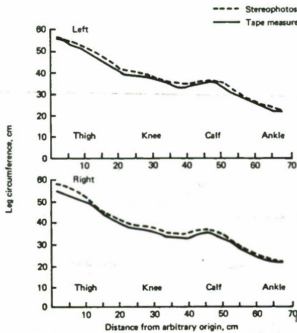
Fig. III-5. Comparison between tape measure and stereometric circumference measurements, ten days preflight, Commander, 3rd Manned Mission. (From ref. III-13, p. 419.)
