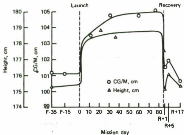
Fig. III-3. Center of gravity/center of mass, Skylab 4 Pilot. (From ref. III-12, p. 650.)
