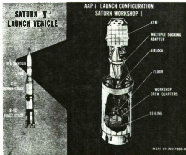
Fig. II-1. Skylab launch configuration and the Saturn V.
