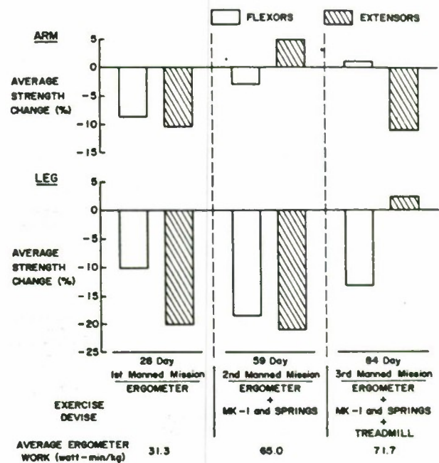
Fig. III-12. Average strength changes. (Modified from ref. III-24, p. 413.)
