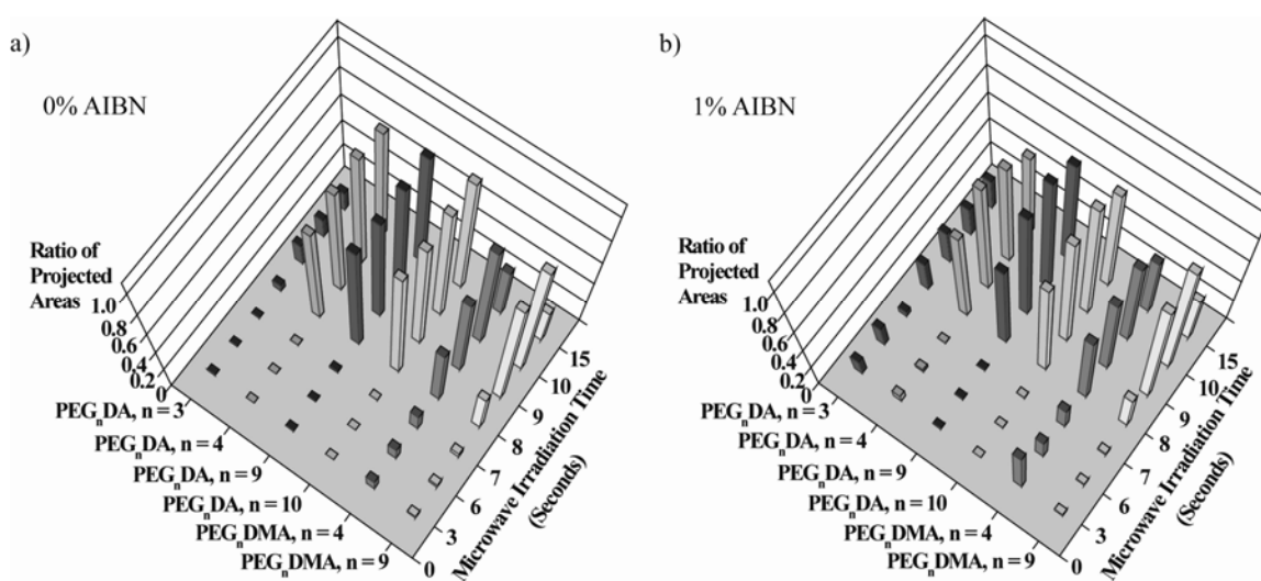
Figure 4. Analysis of crosslinked PEG-based acrylate polymers by using microwave-induced heating. Ratio of projected areas for various PEG n DA (n = 3, 4, 9, 10) and PEG n DMA (n = 4, 9) microarrays with (a) 0% and (b) 1% AIBN.
