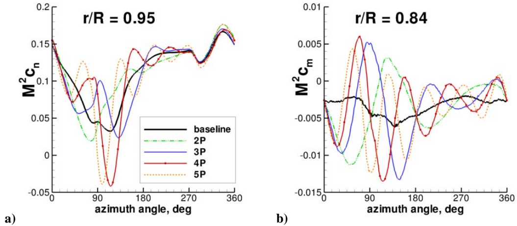
Figure 8. Example airloads a) normal force b) pitching moment with flap input: baseline and 2 – 5/rev, 1.5° deflection, 0° phase, CFD/CSD
