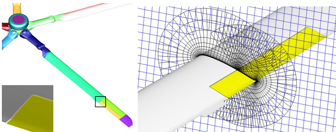
Figure 7. SMART OVERFLOW overset CFD grid system (flap edge inset)
