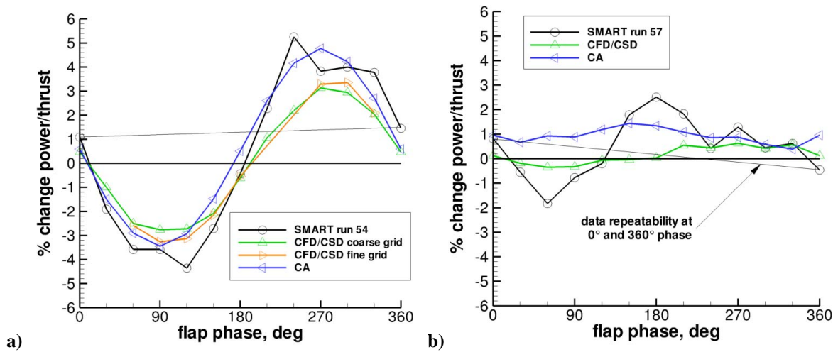
Figure 10. Power/thrust performance increment vs. flap phasing, 2/rev, 1.5° amplitude, varying phase, a) fixed controls, b) trimmed
