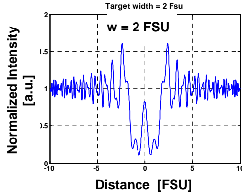
Fig. 6. Occultation intensity profile measured across the center of the shadow for a square satellite with width w = 2 FSU, where 1 \text{ FSU} = \sqrt{\lambda z/2} = 3\text{m} (for z = 36000 \text{ km} and \lambda = 0.5\mu\text{m} ).
