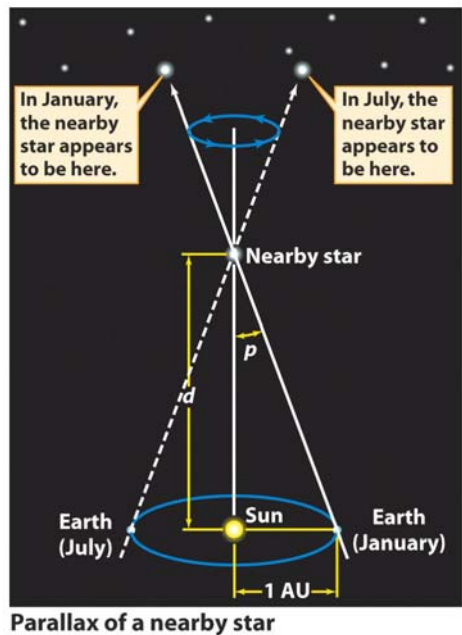
Fig. 2. The astronomical annual parallax to a nearby star is defined as the half-angle of the vertex of a triangle with the orbit of the Earth about the sun as the base. The mean distance of the Earth from the sun is one Astronomical Unit (AU: 149,597,870.69km \pm 0.03km). The annual parallax is thus defined as p = 1\text{AU}/d , where d , the distance to the star, is canonically measured in AU [3]. Similarly, the distance to an Earth-orbiting satellite can be accurately measured if it can be simultaneously observed by two telescopes separated by an accurately known distance, or by modified versions of this basic technique.
