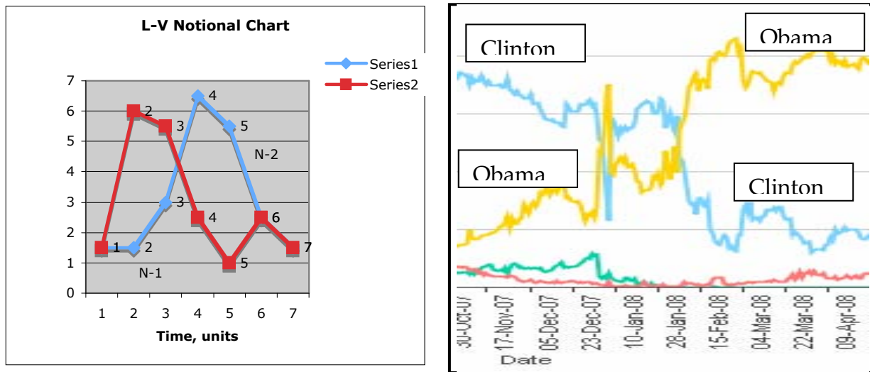
Figure 3. Instead of a limit cycle (i.e., portraying N_1 versus N_2 ; in May, 1973), the data are displayed with N over time, t . Left: The parameters are arbitrary and the result is "frictionless" oscillations. For an interpretation, at time 1 (and t = 3.5, 6 and 7 ), N_1 and N_2 are in direct competition. However, at time 2 (and t = 3, 4 and 5 ), the public has decided to act and social stability reigns. Right: Despite the arbitrary nature of the data on the left, in the campaign to become the Presidential nominee for the Democratic Party, it models the public bets made on the Iowa Electronic Market (IEM; www.biz.uiowa.edu/iem/index.cfm ) in support of Clinton and Obama during a brief period of intense competition (during January 2008), followed by the IEM public's later decision to favor Obama (by February 2008). 27 (Postponed for future consideration is whether these data, already normalized, need to be further de-trended; see Turchin, 2005)
