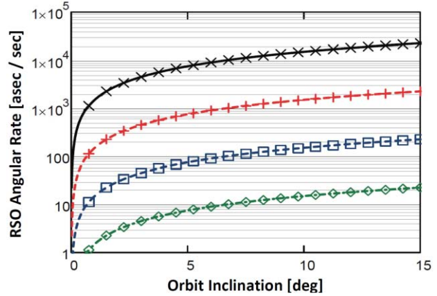
Figure 12 The angular rates of GEO RSOs crossing zero declination as a function of orbital inclination (x axis). Rates are shown for objects having GEO angle differences of 0.01° (X), 0.1° (+), 1° (□) and 10° (◇).
