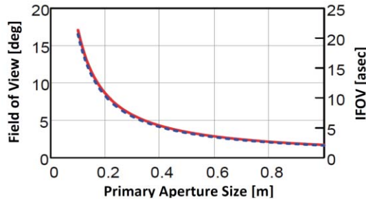
Figure 6 The field of view (left y-axis) and instantaneous field of view (right y-axis) as a function of aperture size for an f/\# 1.2 optical system with a 36 mm CCD having 12 \mu\text{m} pixels.
