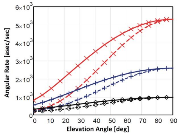
Figure 7 A range of LEO RSO angular velocities as seen from the ground are shown as a function of elevation angle. Circular orbit altitudes of 300 km (X), 600 km (+) and 1500 km (◇) are provided, with solid lines representing the maximum angular velocity, and the dotted lines the minimum.
