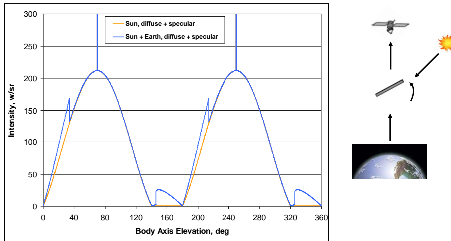
Fig. 11. Total LEO and GEO Signatures for Nadir View of a Tumbling Plate
