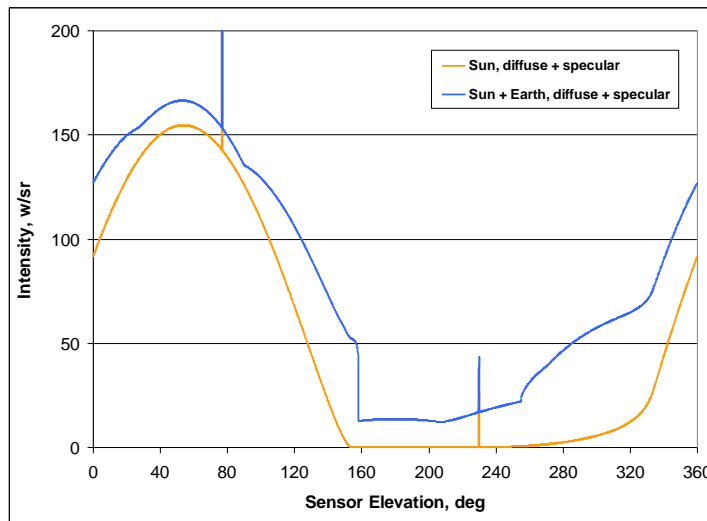
Fig. 6b. Total LEO and GEO Signatures for a Horizontal-Pointing Cone
