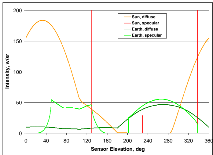
Fig. 8a. Signature Components for a Zenith-Pointing Frustum
