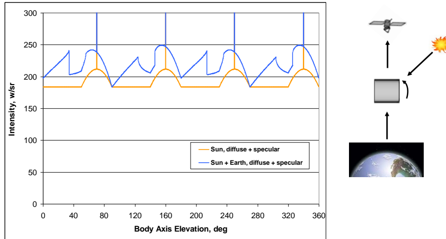
Fig. 10. Total LEO and GEO Signatures for Nadir View of a Tumbling Cylinder
