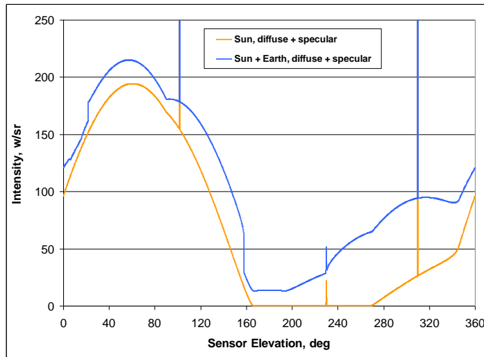
Fig. 9b. Total LEO and GEO Signatures for a Horizontal-Pointing Frustum
