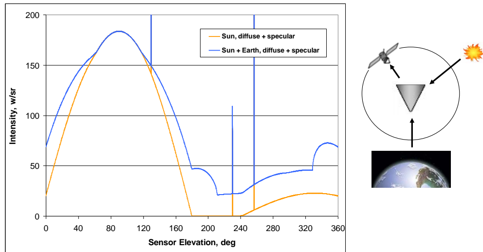
Fig. 4b. Total LEO and GEO Signatures for a Nadir-Pointing Cone
