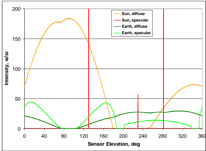
Fig. 7a. Signature Components for a Nadir-Pointing Frustum
