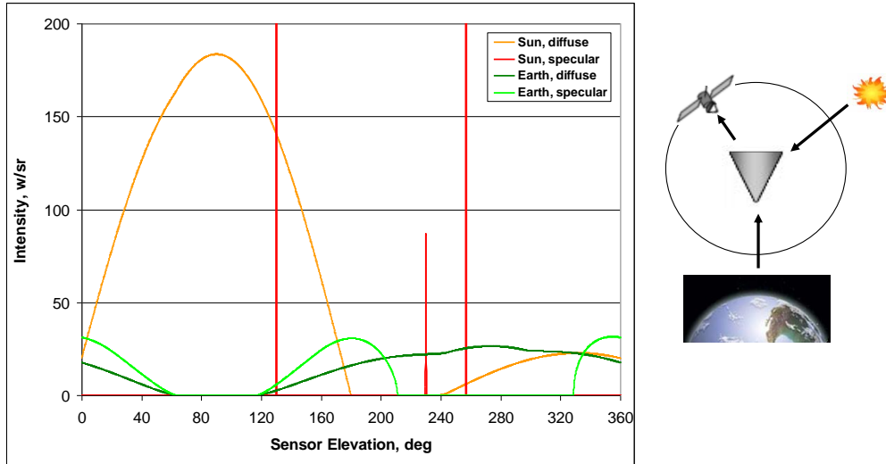
Fig. 4a. Signature Components for a Nadir-Pointing Cone
