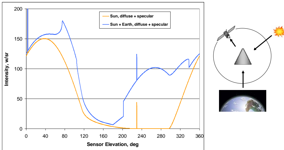
Fig. 5b. Total LEO and GEO Signatures for a Zenith-Pointing Cone
