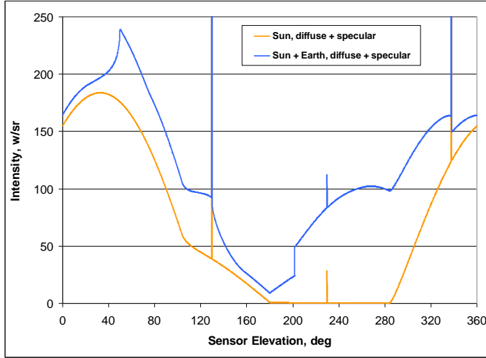
Fig. 8b. Total LEO and GEO Signatures for a Zenith-Pointing Frustum
