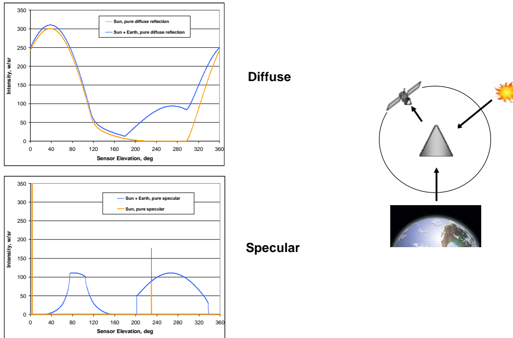
Fig. 12. Total LEO and GEO Signatures for Zenith-Pointing Pure Diffuse and Pure Specular Cones
