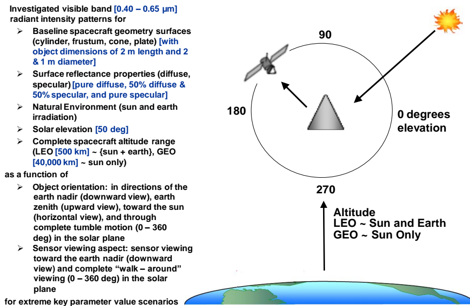
Fig. 2. Process and Parameters Used To Generate Signature Database
