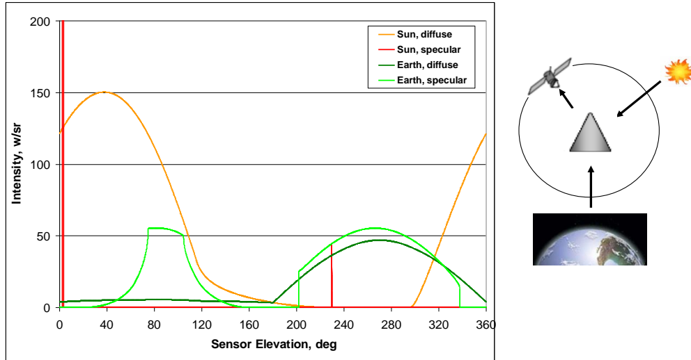
Fig. 5a. Signature Components for a Zenith-Pointing Cone
