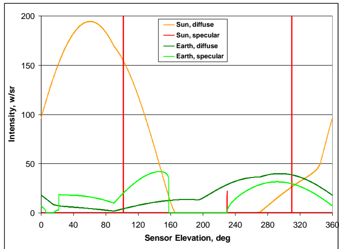
Fig. 9a. Signature Components for a Horizontal-Pointing Frustum
