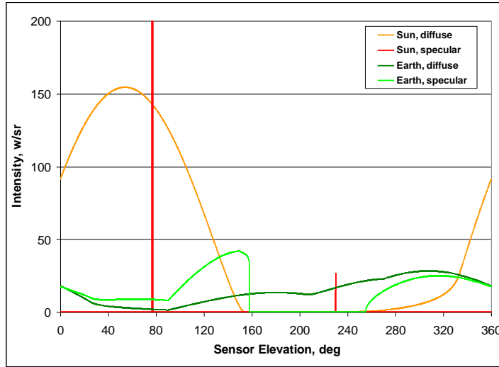
Fig. 6a. Signature Components for a Horizontal-Pointing Cone
