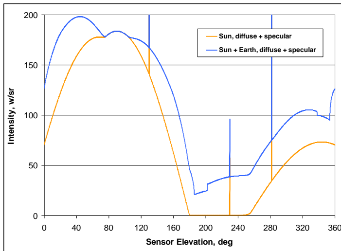
Fig. 7b. Total LEO and GEO Signatures for a Nadir-Pointing Frustum
